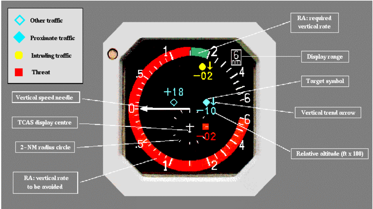
Figure 3. TCAS RA Display Implemented on an IVSI
